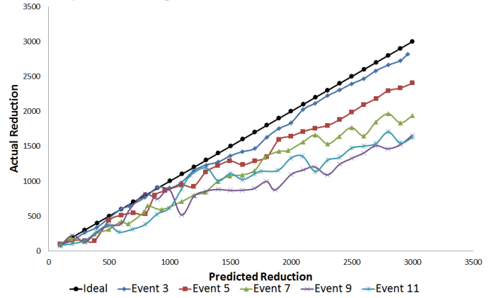
Fig. 7: Comparison of predicted to achieved reduction with stable window=2 size.
