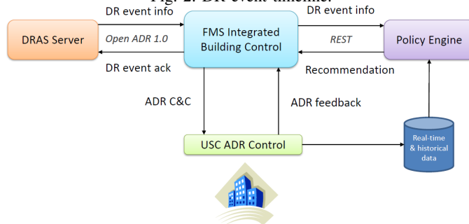
Fig. 3: Overview of the existing integrated platform for ADR.
