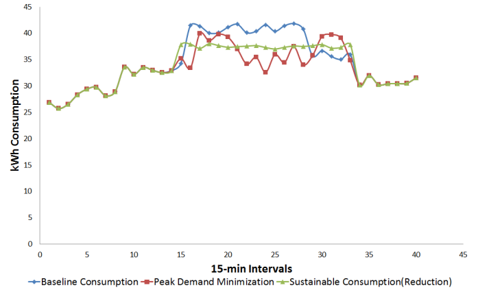
Fig. 1: Sustainable reduction compared to peak minimization.
